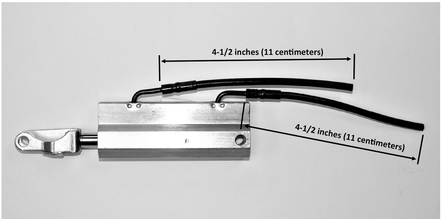
Cylinder orientation for 2004-2010 Mercedes-Benz SLK-Class (R171 chassis) as seen while sitting in the car and looking up, P/N 1718000072.
