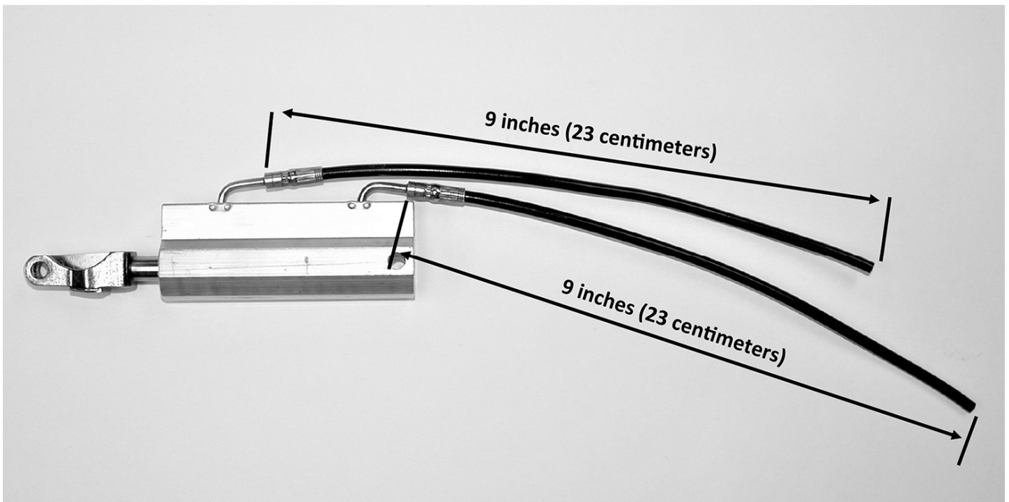
Cylinder orientation for 1998-2004 Mercedes-Benz SLK-Class (R170 chassis) as seen while sitting in the car and looking up, P/N 1708000072.
